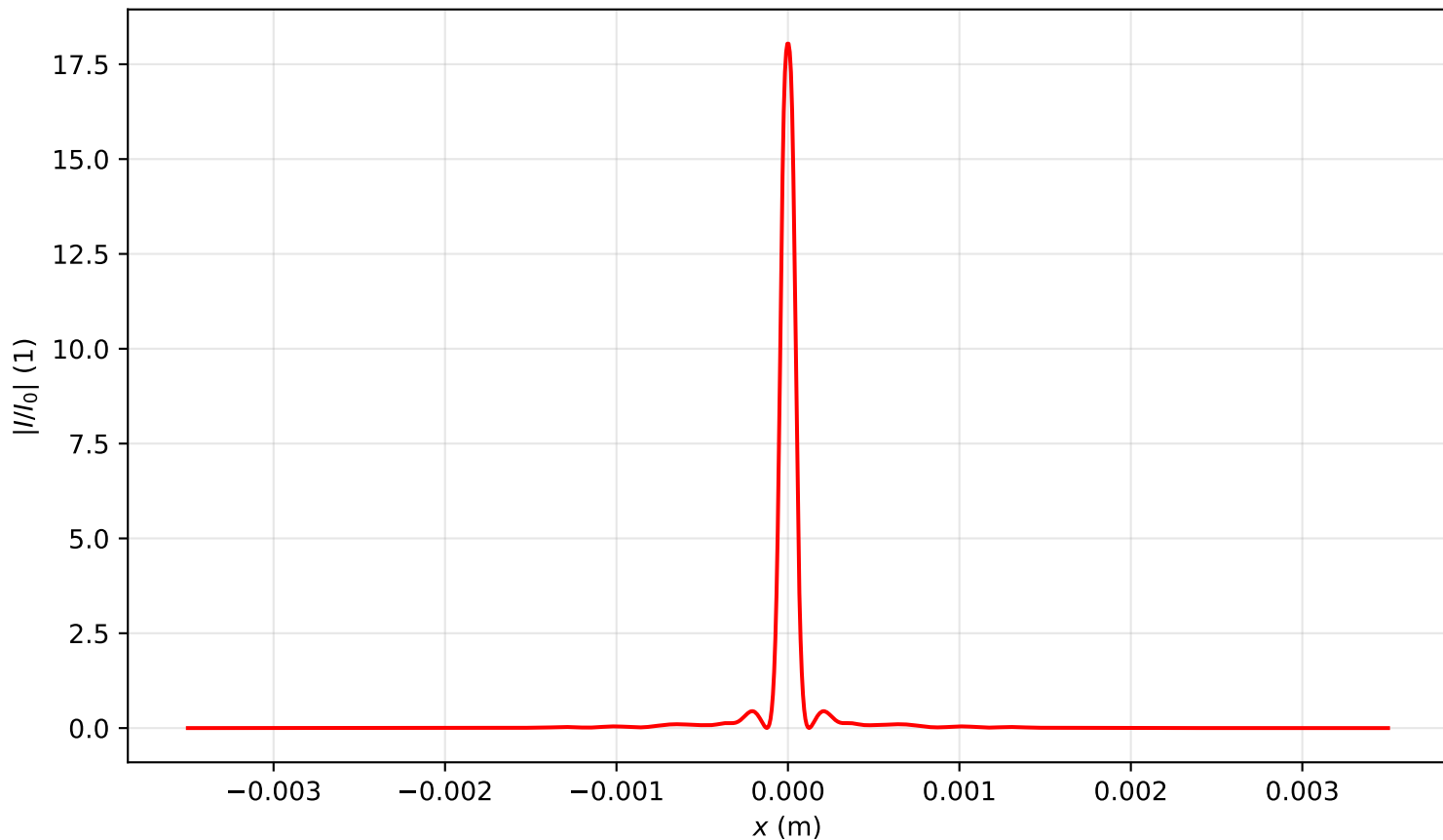
Intensity profile I(x, y = 0, z = 1.433)/I_0 , P_{in}=6.0P_{cr} , artificial time
